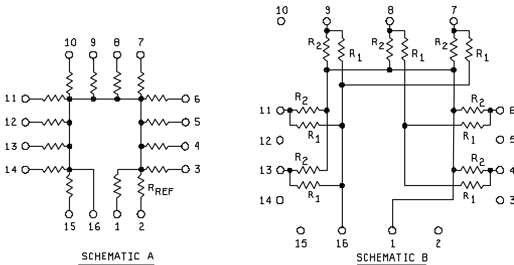
FIGURE 1. Schematics .
