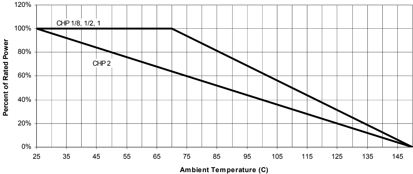
CHP POWER DERATING CURVE
