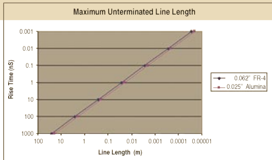
Fig. 1. Maximum physical lengths of unterminated transmission lines.
