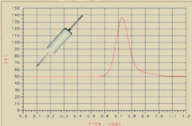
Fig. 7b. Axial-leaded RN55.
