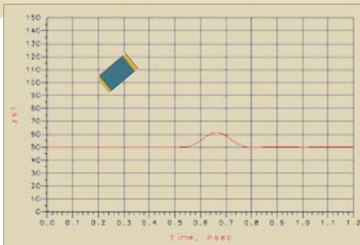
Fig. 7c. PFC 0603 chip.
